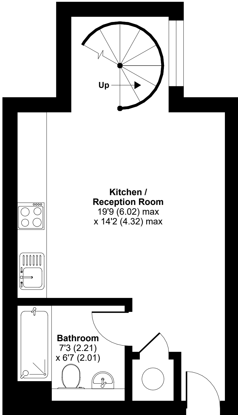
GROUND FLOOR
