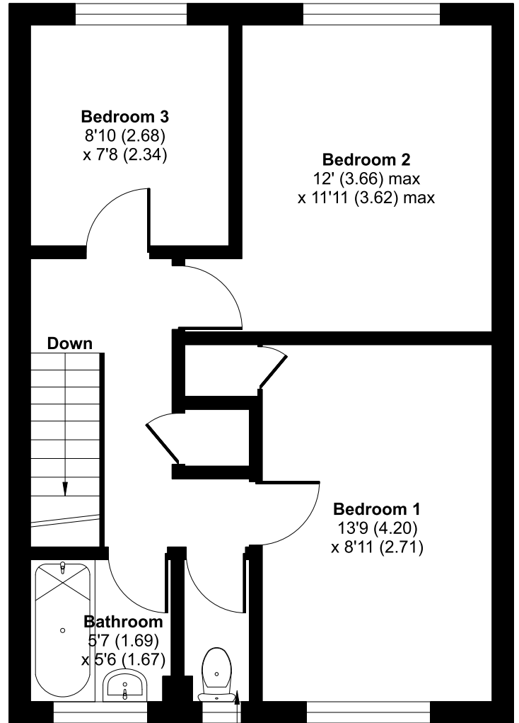
SECOND FLOOR
